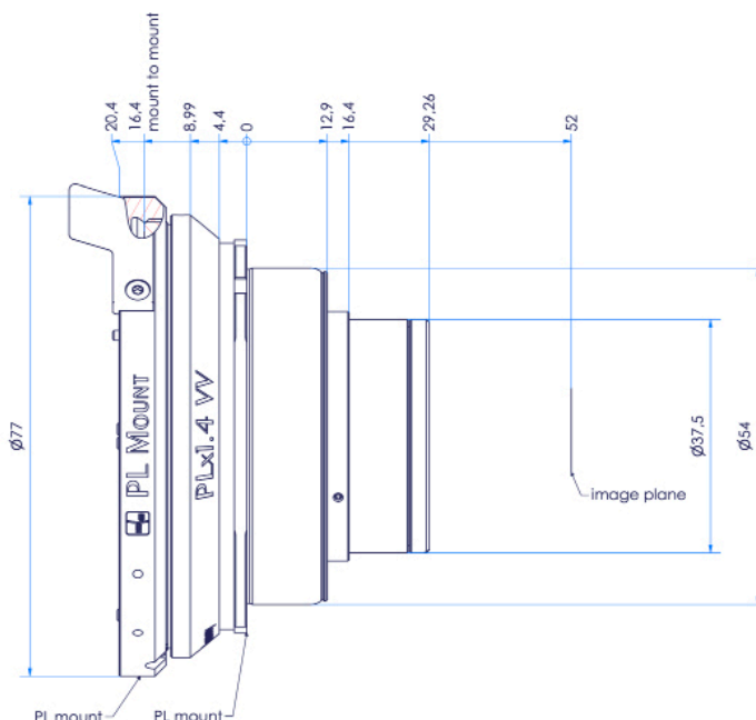
III. 2: dimensional drawing
